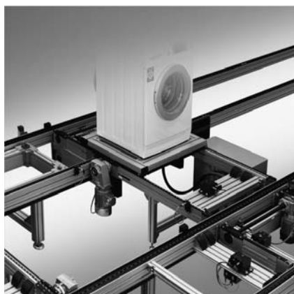
TS 4plus (250 kg)
